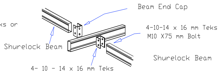
BEAMS TO INTERNAL BEAM Detail No. 6
