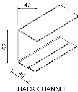
BACK CHANNEL
