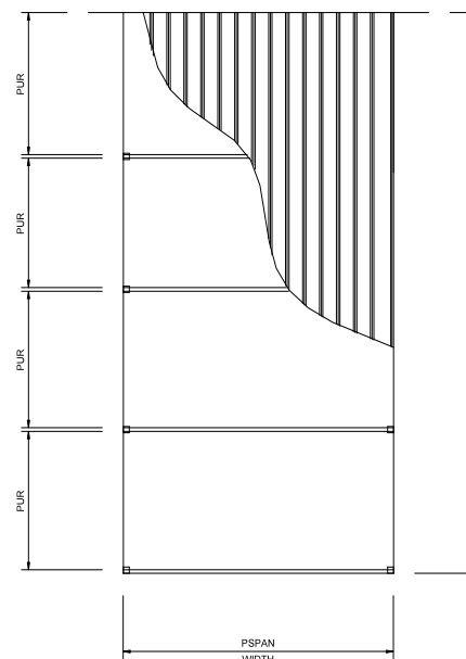
Attached Car Port/Patio No Edge Beams Fig 5
