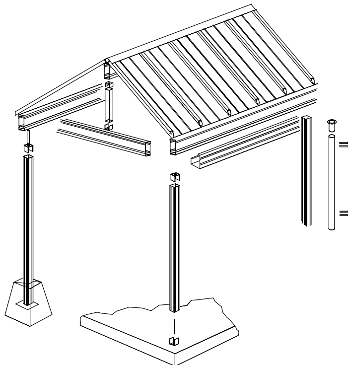
GF2 GABLE FRAME
