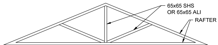
GF2 GABLE FRAME
