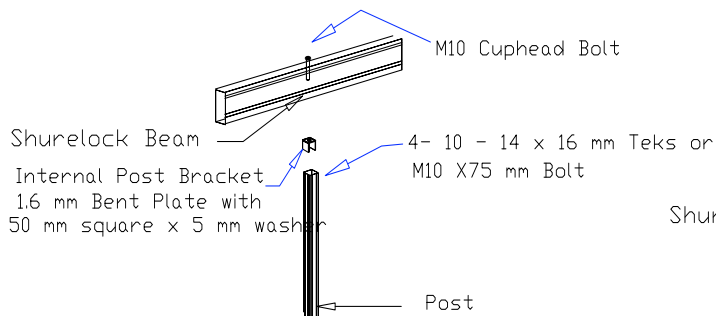
Beam to Post Connection Detail Detail No. 5
