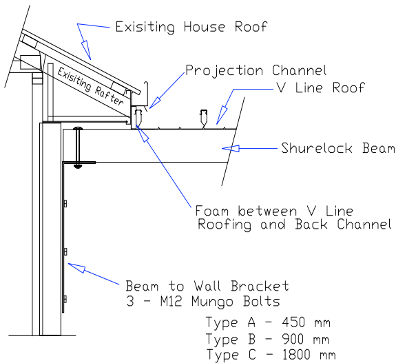
Beam to Wall Bracket Detail Detail No. 1
