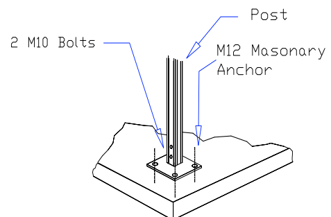
External Footing Bracket Detail No. 4 (not suitable for freestanding)
