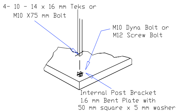
Internal Footing Bracket Detail No. 3 (Not suitable for freestanding)
