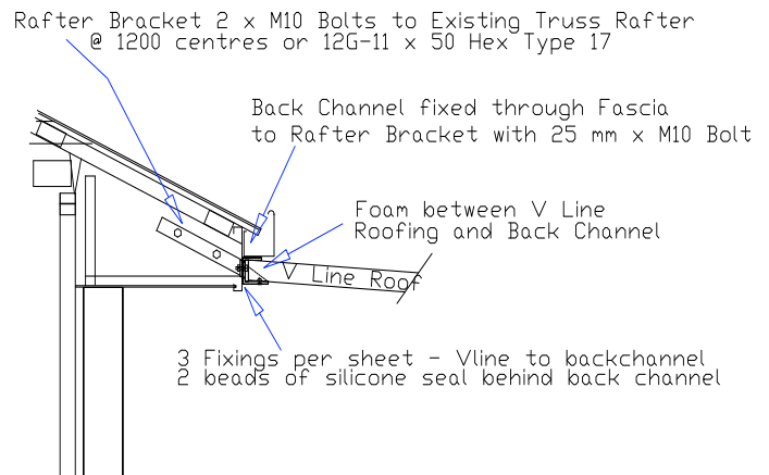
Rafter Bracket to Backchannel Detail Detail No. 2
