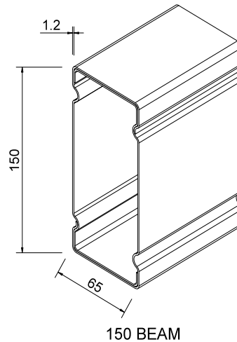
150 BEAM
