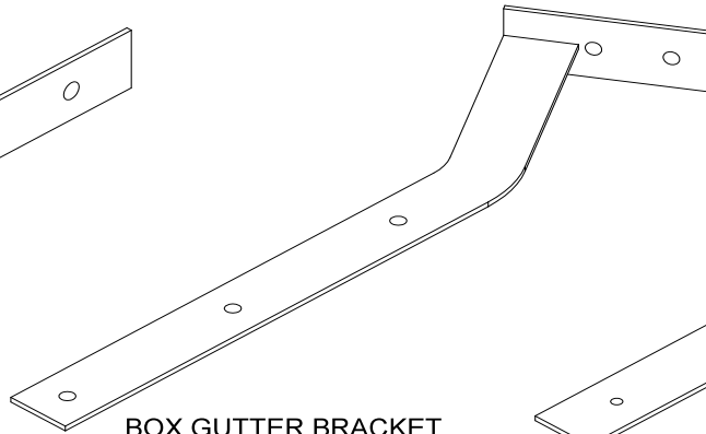
BOX GUTTER BRACKET
