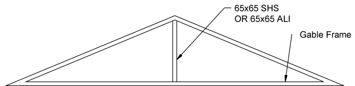
Non - Cyclonic Gable
