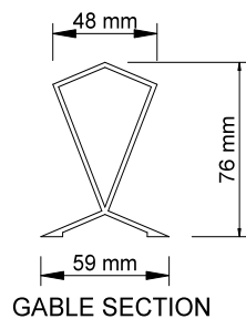
GABLE SECTION
