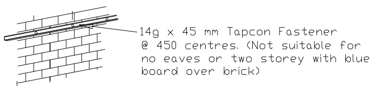
BACK CHANNEL TO WALL Detail No:13
