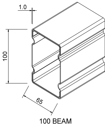
100 BEAM
