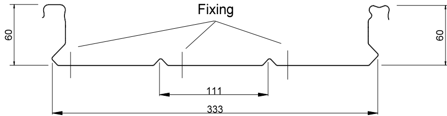
V-LINE ROOF SHEET
